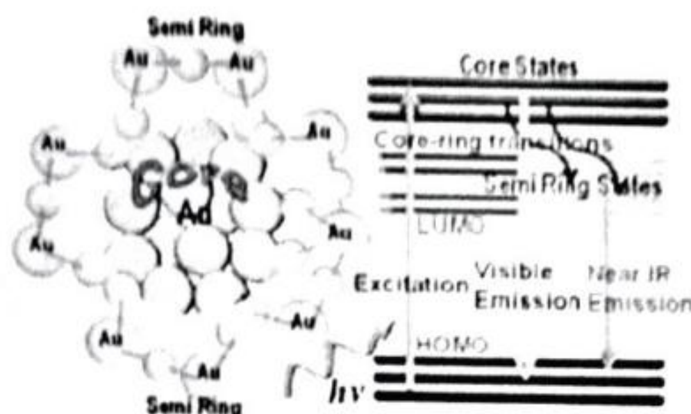
Core and CT type states for Au_{25}SR_{18} clusters, with different excited state lifetimes
